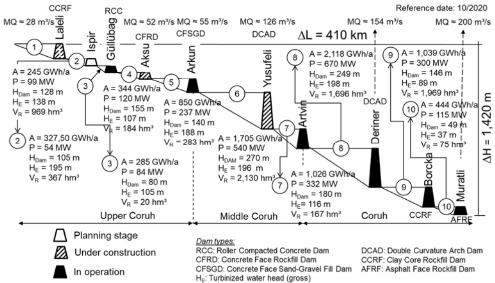
Fig. 1. Development of hydro on the Çoruh river (adapted from Haselsteiner et al., 2012; after Sezer, 2009; and after Sucu & Dinc, 2008)
