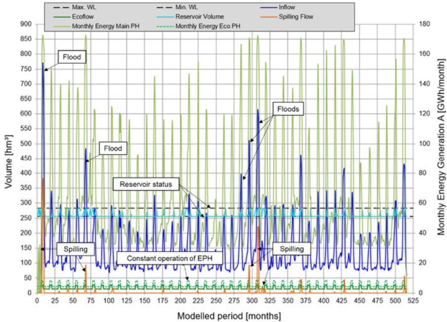
Fig. 4. Output diagram for the modelled period of 516 months showing monthly flows and production values (scheme 6, see Table 1)
